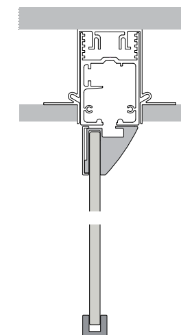
CONTROBINARIO A SOFFITTO Counter-beam ceiling rail
