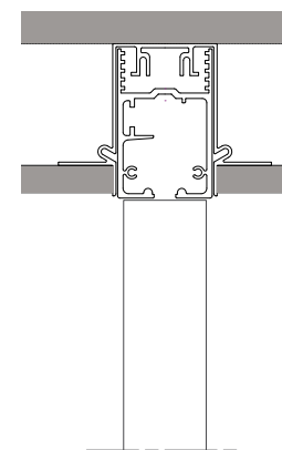
CONTROBINARIO A SOFFITTO Counter-beam ceiling rail
