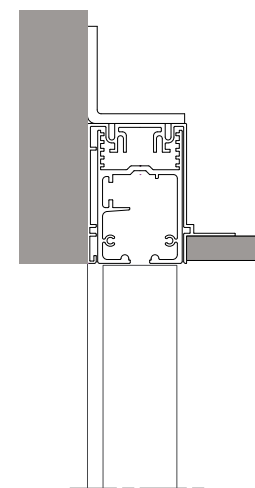
CONTROBINARIO A PARETE Counter-beam wall rail
