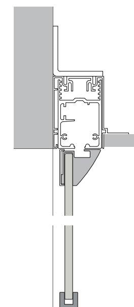
CONTROBINARIO A PARETE Counter-beam wall rail
