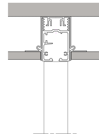
CONTROBINARIO A SOFFITTO Counter-beam ceiling rail
